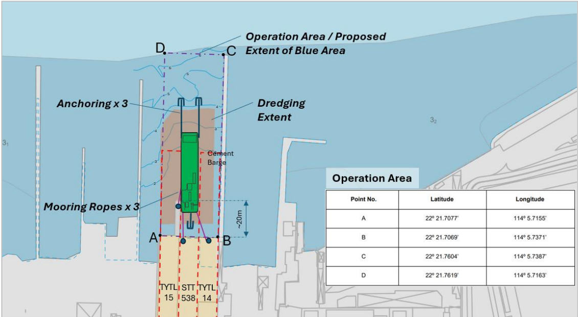
Figure 5.3 Mooring Arrangement of Cement Barge
