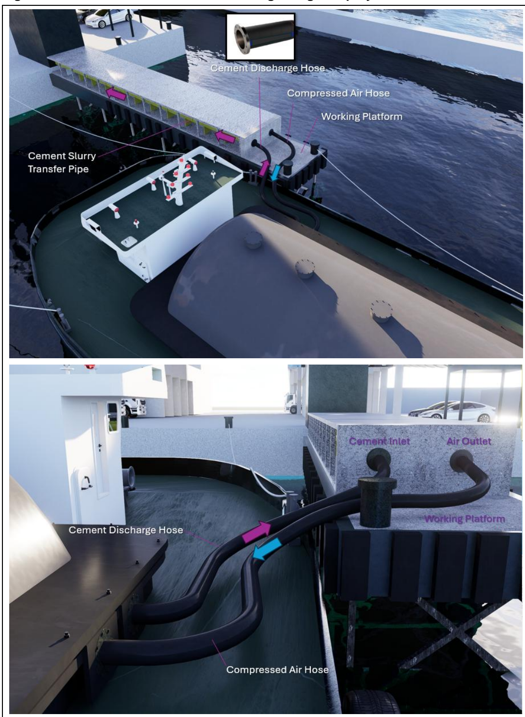
Figure 6.2 Illustration of Cement Unloading Using Pump System
