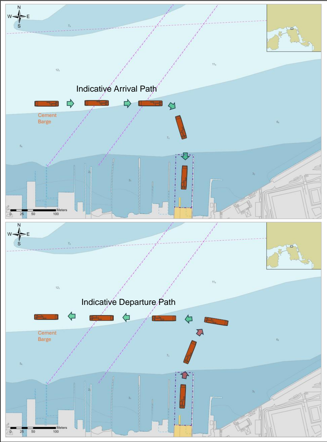
Figure 6.4 Example of Arrival and Departure Path of Cement Barge
