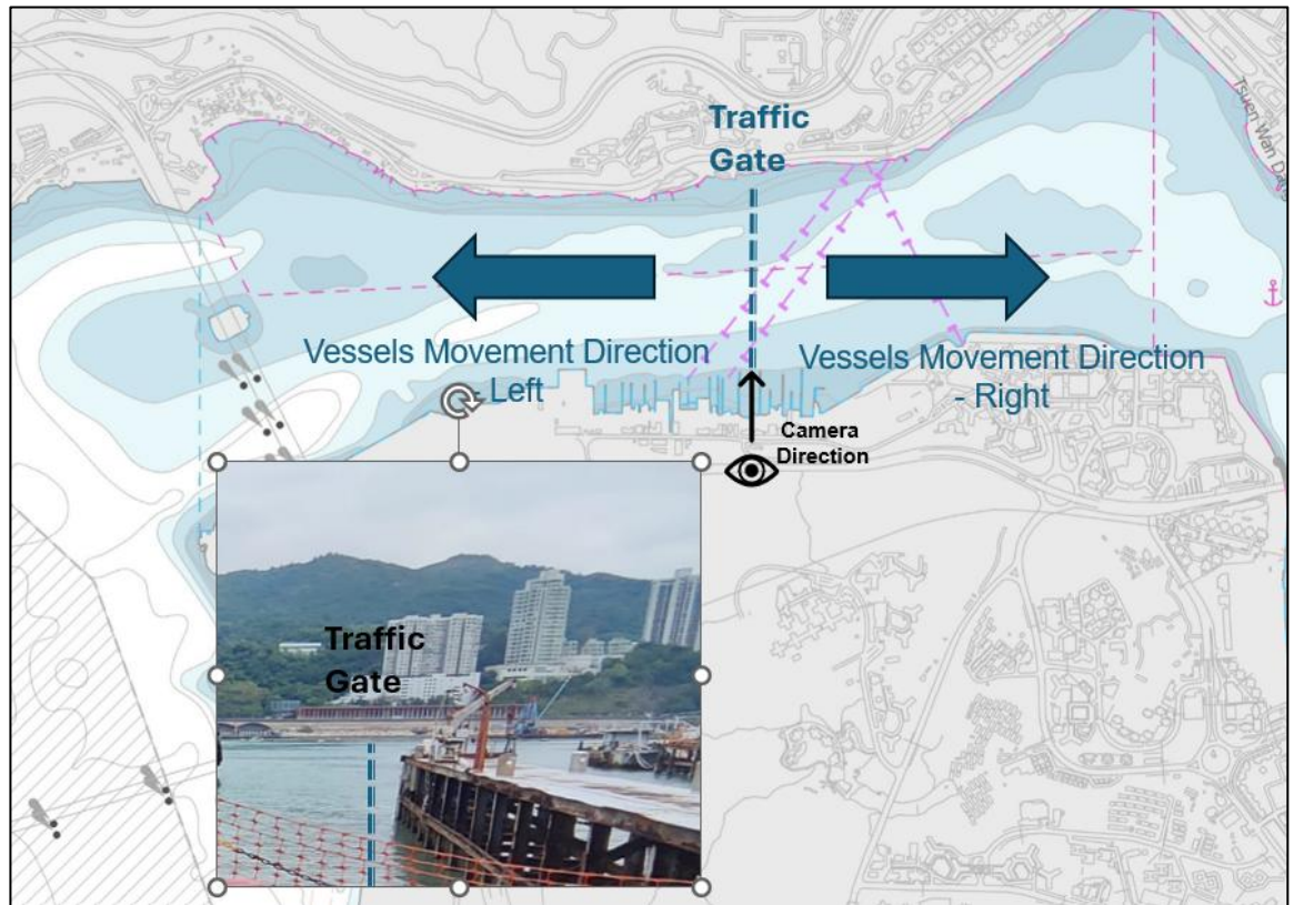
Figure 7.6 Traffic Gate and Vessels Movement Direction
