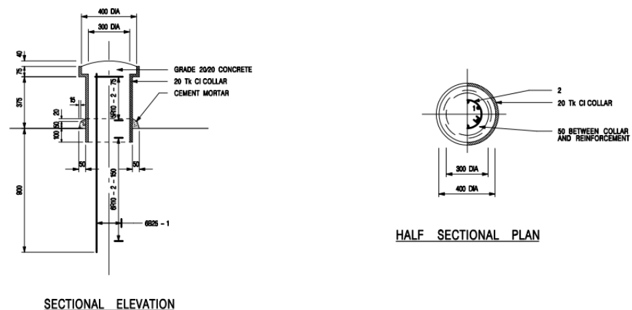
Figure 5.4 Typical Arrangements of Mooring Bollard
