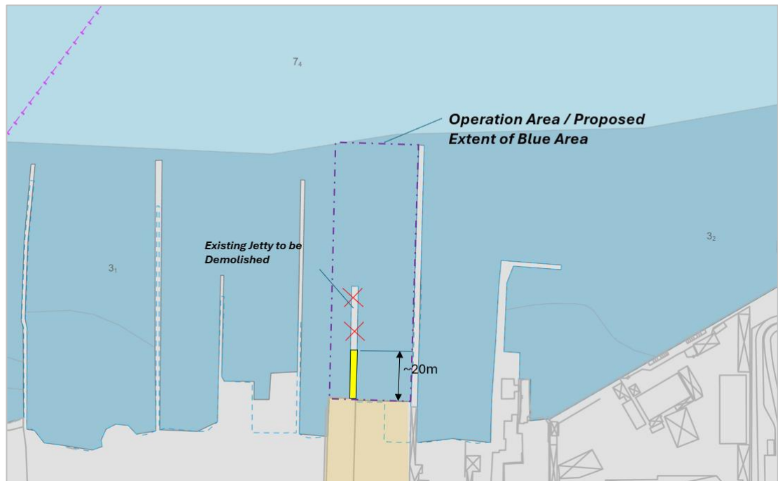
Figure 5.1 Proposed Improvement of Safety Platform
