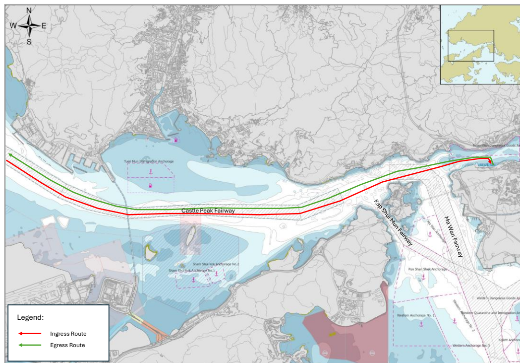
Figure 3.1 Proposed Delivery Routes
