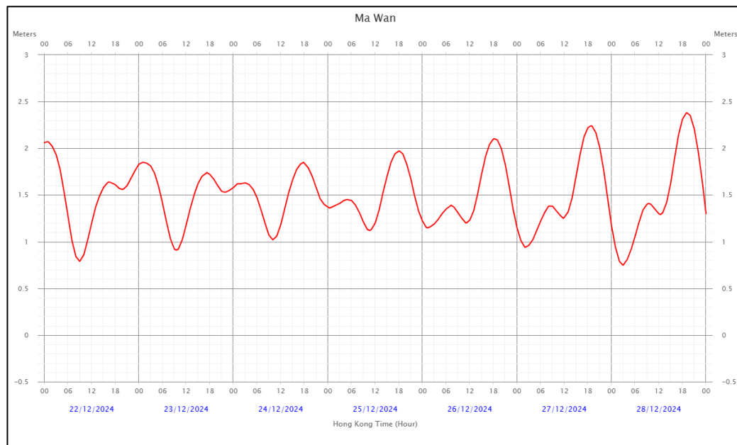
Figure 7.3 Sample of Predicted Tides for Ma Wan
