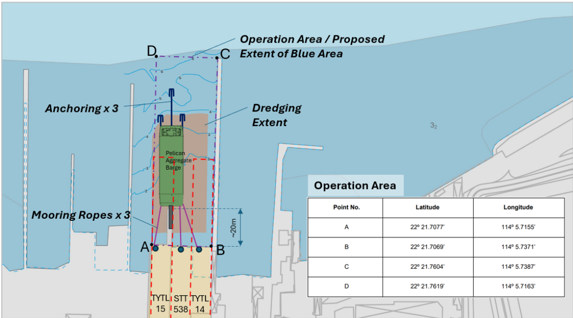
Figure 5.2 Mooring Arrangement of Pelican Aggregate Barge
