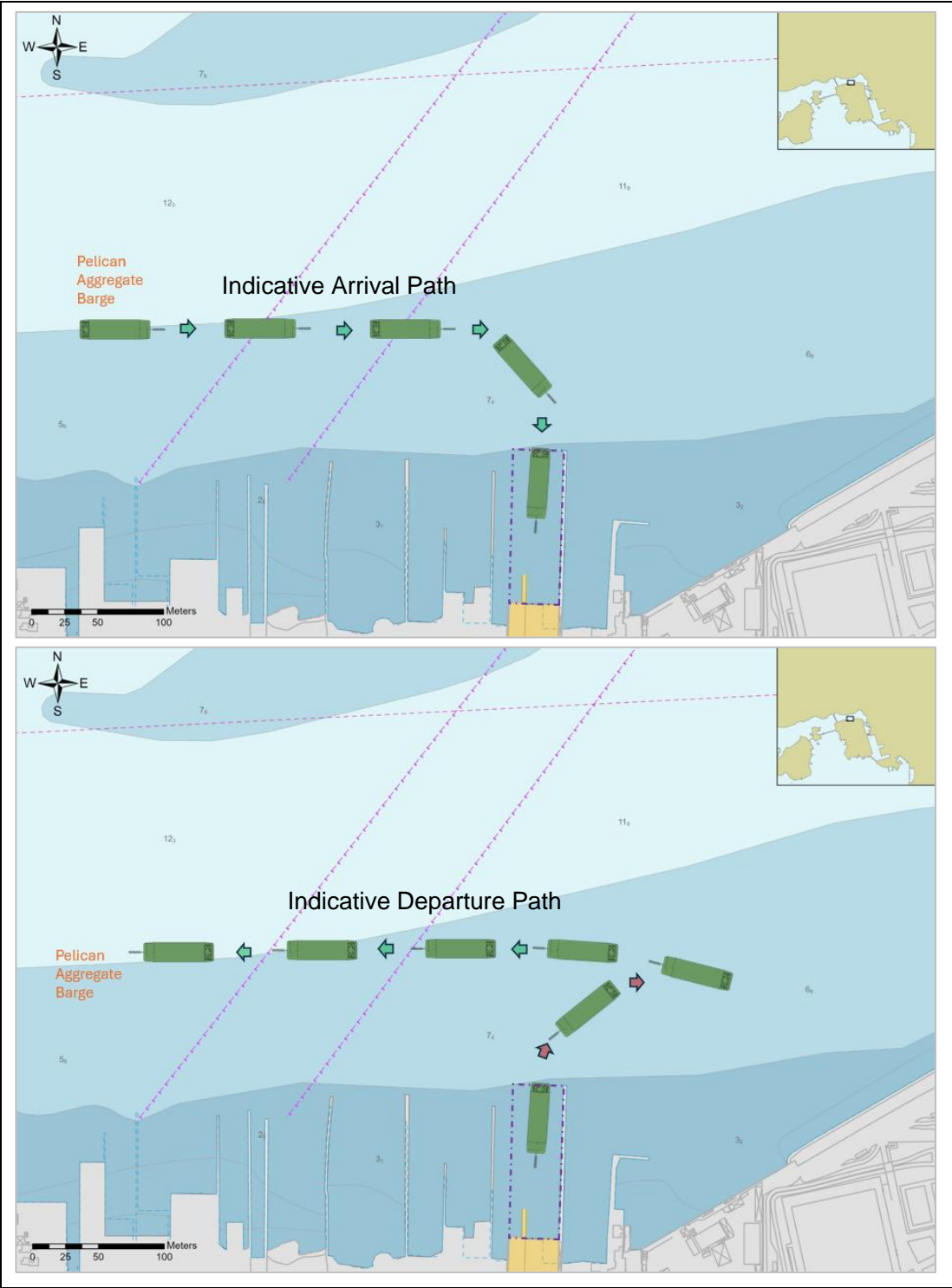
Figure 6.3 Example of Arrival and Departure Path of Pelican Aggregate Barge
