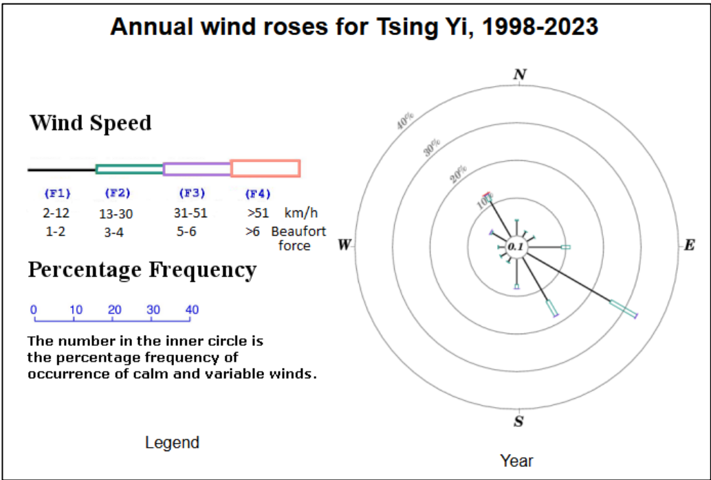
Figure 7.2 Annual Wind Rose for Tsing Yi, 1998-2023
